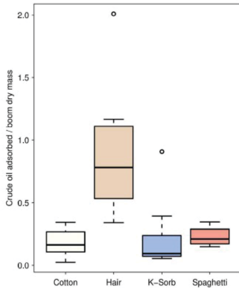
Fig. 1. Crude oil adsorbed (per gram of sorbent) compared across boom types.
