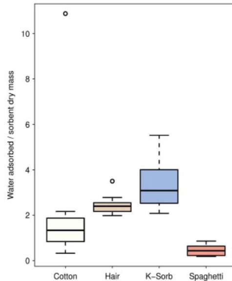
Fig. 3. Water adsorbency ratio compared across inner sorbents.
